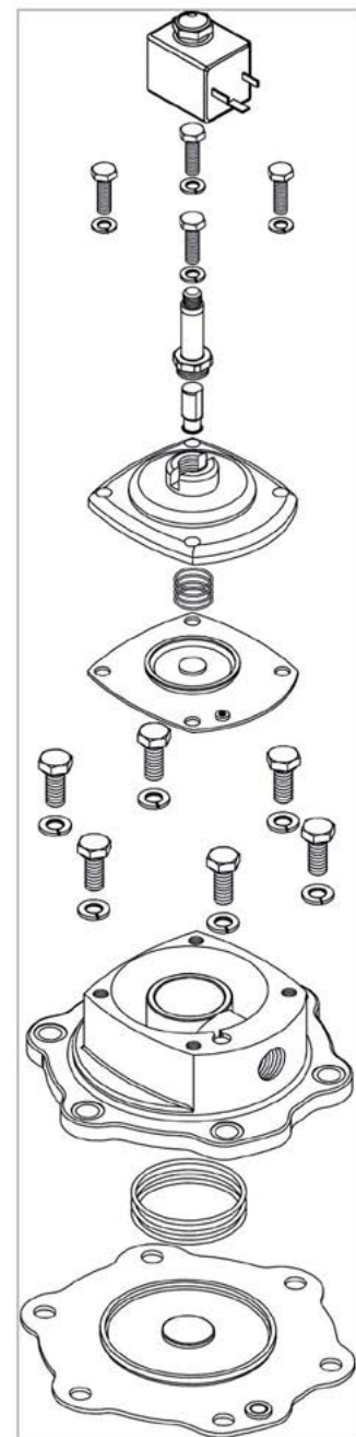
Exploded view of SV-150
