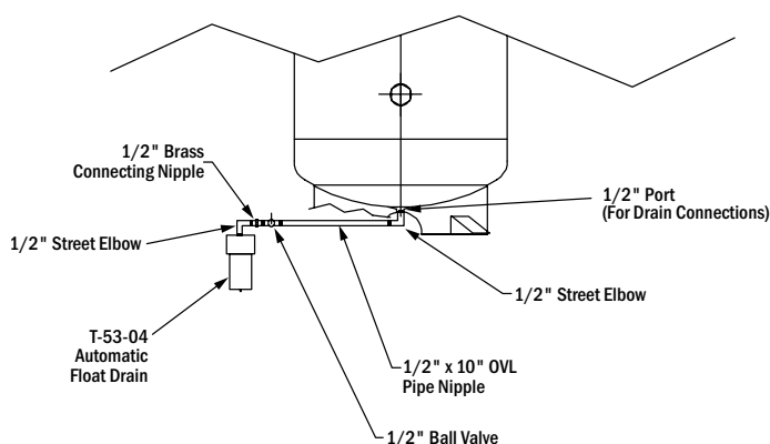
Air Receiver Float Drain Connection Details
